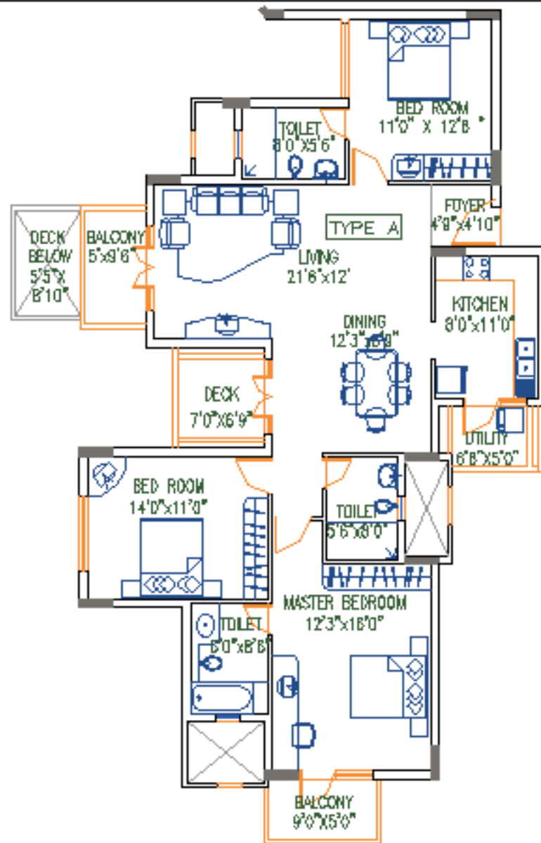
TYPICAL FLOOR PLAN
